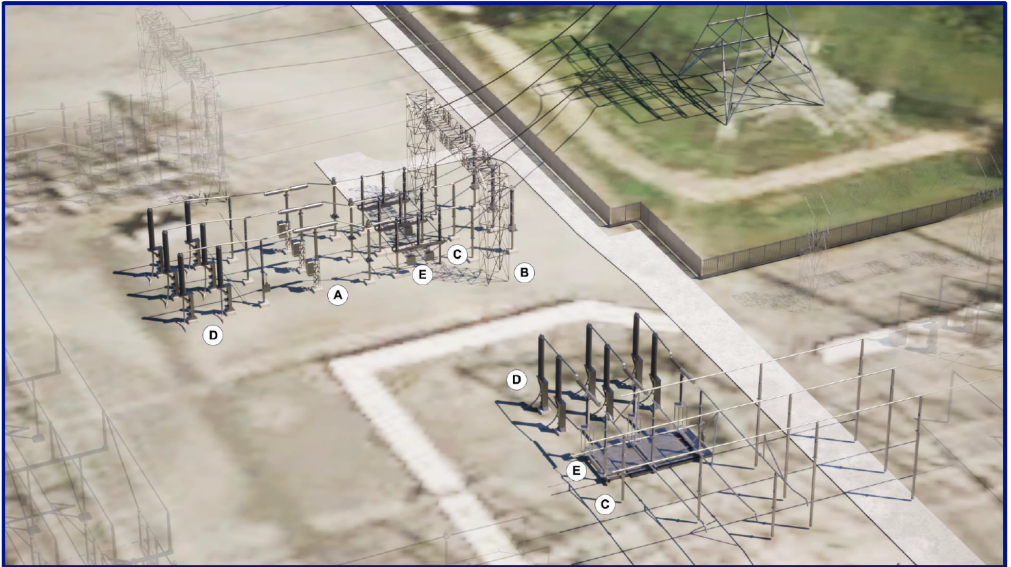
Figure 14: Osbaldwick Substation Illustration Labelled (as detailed in Key at 3.2.6 above)
