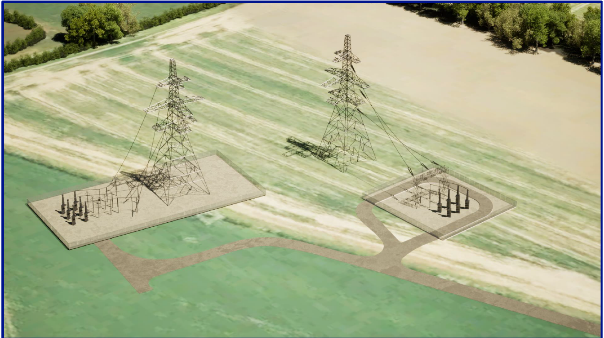
Figure 15: Shipton Cable Sealing End Compounds Illustration
